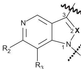
5-Aza-Derivate
